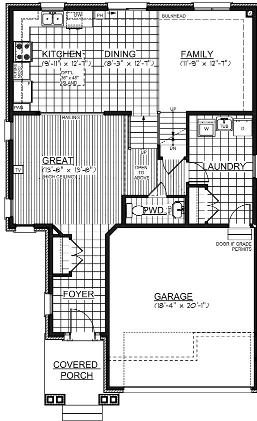
MAIN FLOOR PLAN SQ. FT. = 1020
