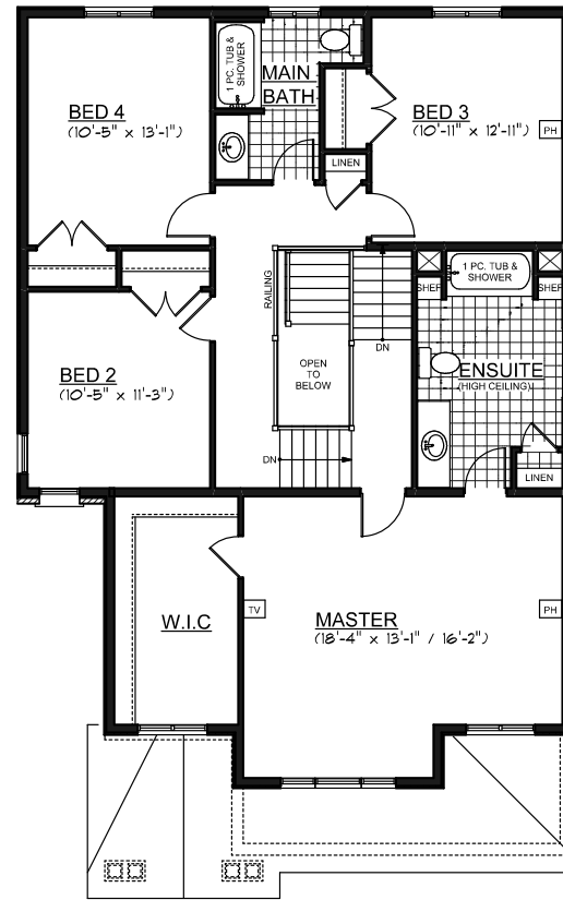
SECOND FLOOR PLAN GROSS SQ. FT. = 1315 DEDUCT O.T.A. SQ. FT. = 42 NET SQ. FT. = 1273
