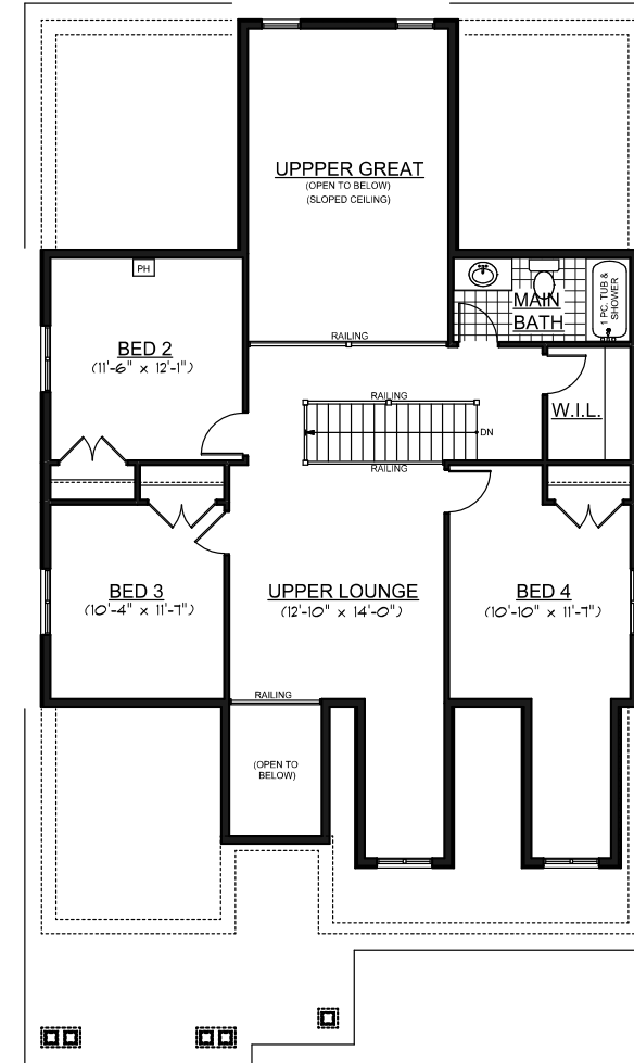
SECOND FLOOR PLAN GROSS SQ. FT. = 1346 DEDUCT O.T.A. SQ. FT. = 344 NET SQ. FT. = 1002
