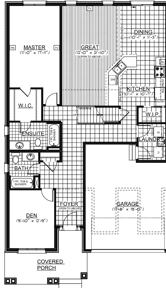
MAIN FLOOR PLAN SQ. FT. = 1539
